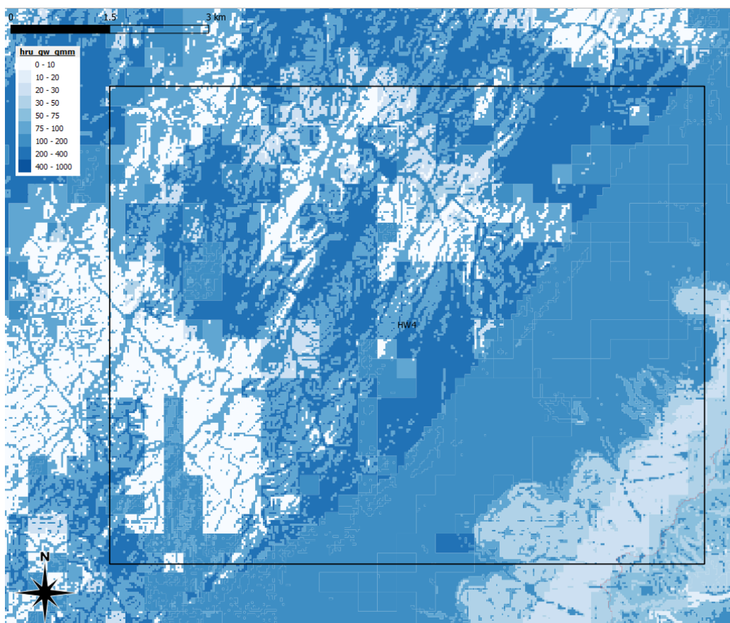
Figure 6.24. Spatial variation of the annual average groundwater recharge amounts [mm y -1 ] in the HW4 target area over the 1994-2013 period.
