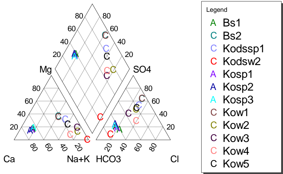
Figure 8.3. Piper plot for the existing water sources in target area HW34.
