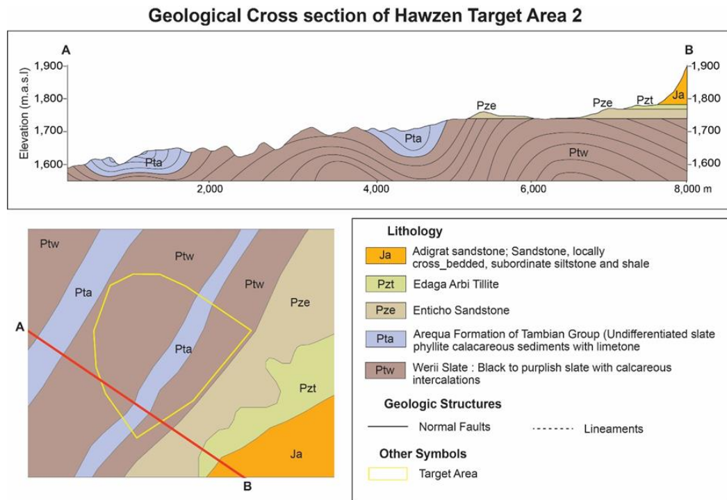
Figure 4.4. Geological cross section across target area 2 of the Hawzen Woreda.
