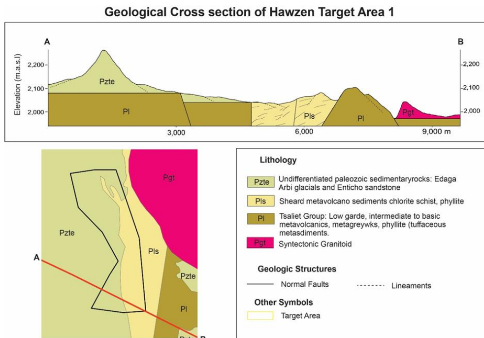
Figure 4.2. Geological cross section of target area 1 of the Hawzen Woreda.
