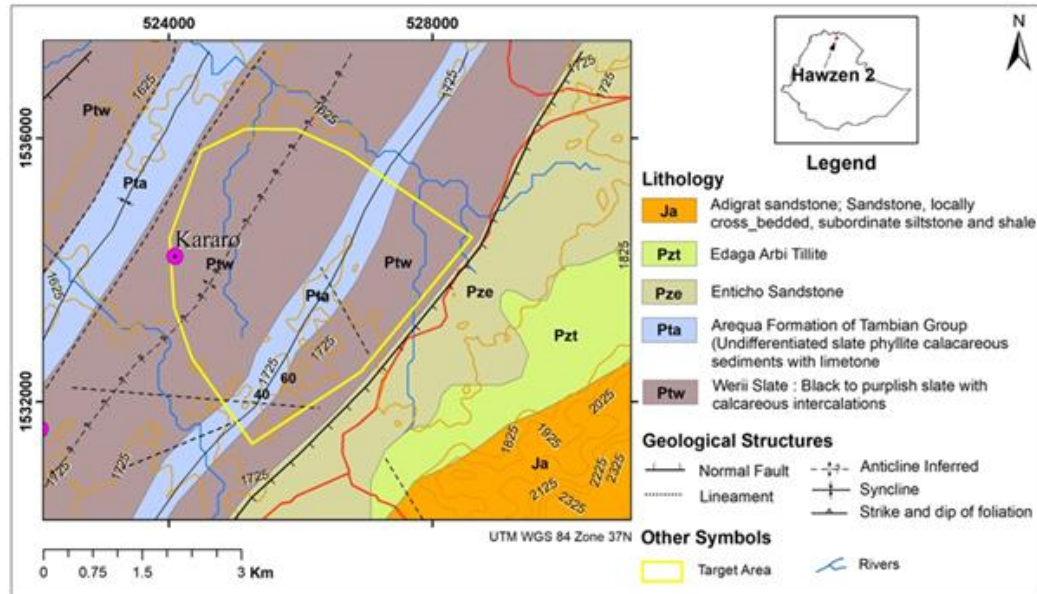
Figure 4.3. Geological map of target area 2 of the Hawzen Woreda.
