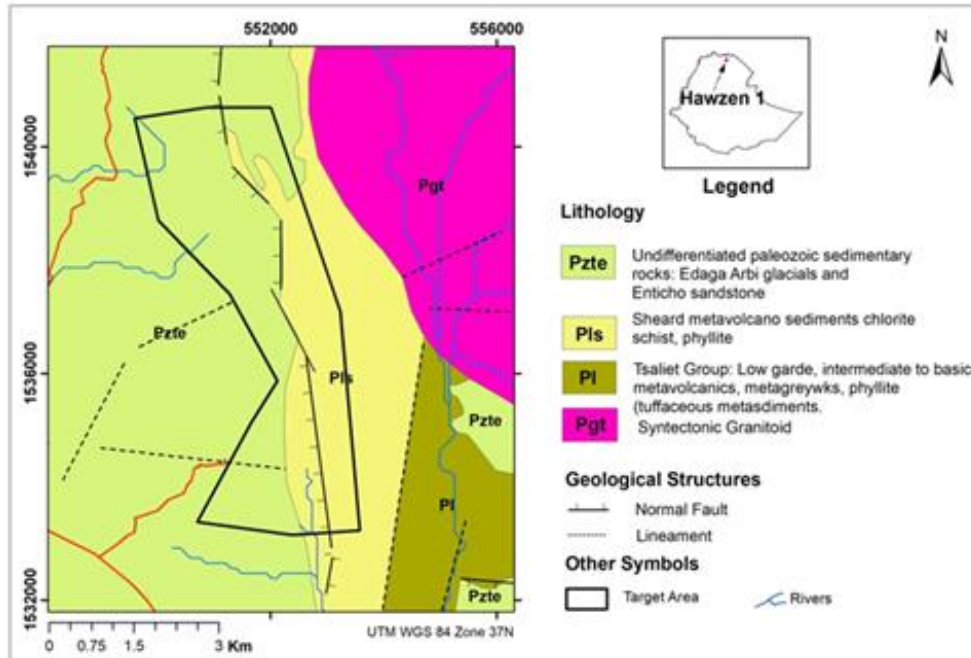
Figure 4.1. Geological map of target area 1 of the Hawzen Woreda.
