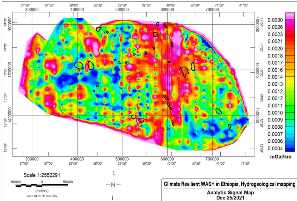
Figure 5.9. Analytical signals.
