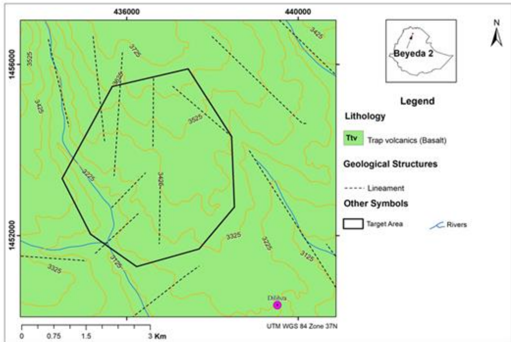
Figure 4.3. Geological map of target area 2 of the Beyeda Woreda.
