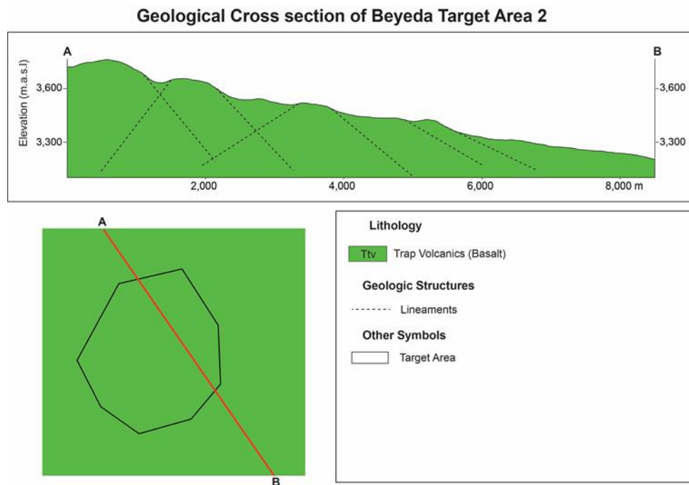
Figure 4.4. Geological cross section across target area 2 of the Beyeda Woreda.
