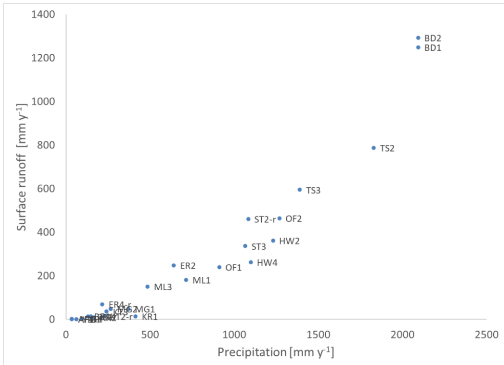
Figure 6.25. Relation between annual average precipitation and river runoff for the various target areas.
