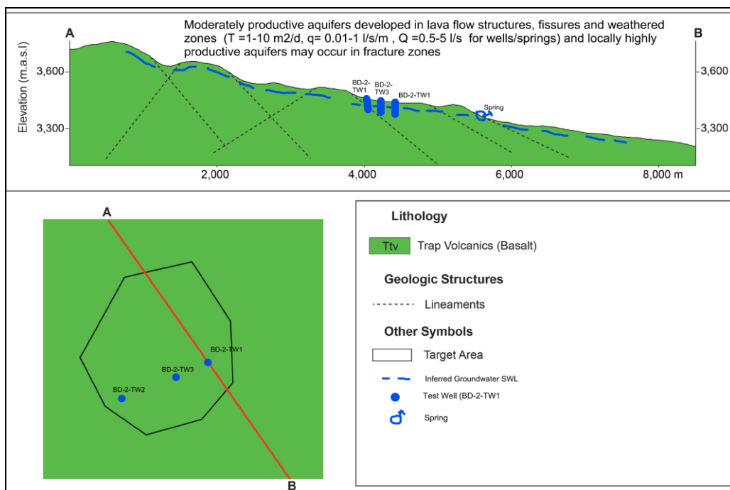
Figure 7.2. Conceptual model for target Beyeda BD-2.
