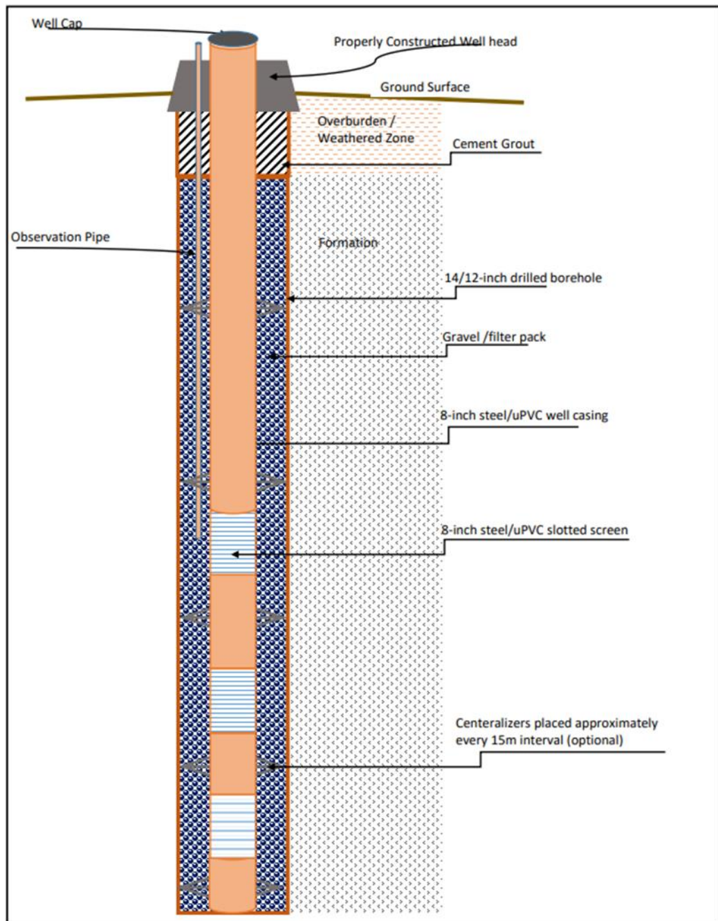
Figure 9.1. Generic well design for Beyeda woreda.
