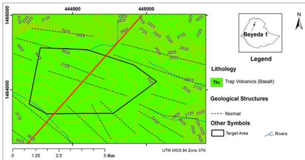
Figure 4.1. Geological map of target area 1 of the Beyeda Woreda.
