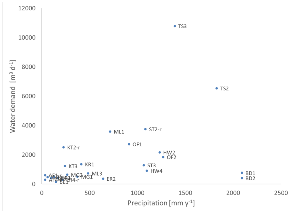
Figure 6.27. Relation between annual average precipitation and estimated target area total water demands.
