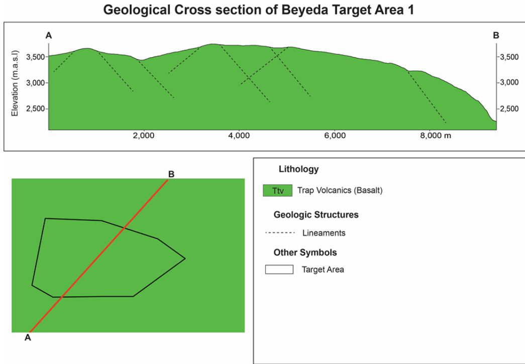
Figure 4.2. Geological cross section of target area 1 of the Beyena Woreda.
