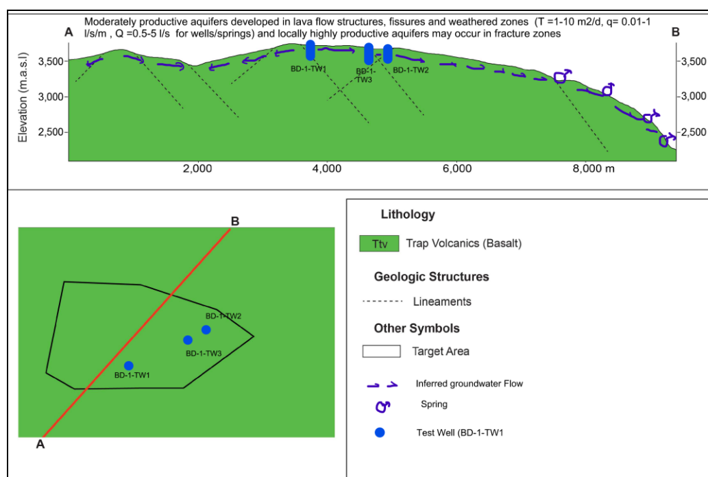
Figure 7.1. Conceptual model for target area Beyeda BD-1.
