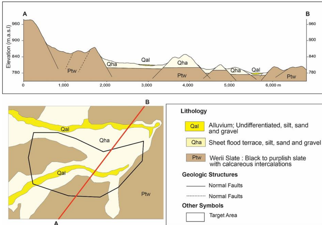
Figure 4.4. Cross section across the target area 2 (Berehale Woreda). Inset shows line of cross sections
