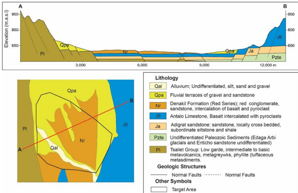
Figure 4.2. Cross section across the target area 1 (Berhale). Line of cross section is shown in the inset.
