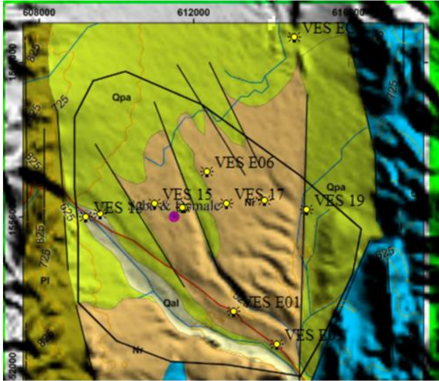
Figure 5.17. Map showing the positions of VES points within BE4r of Berehale woreda.
