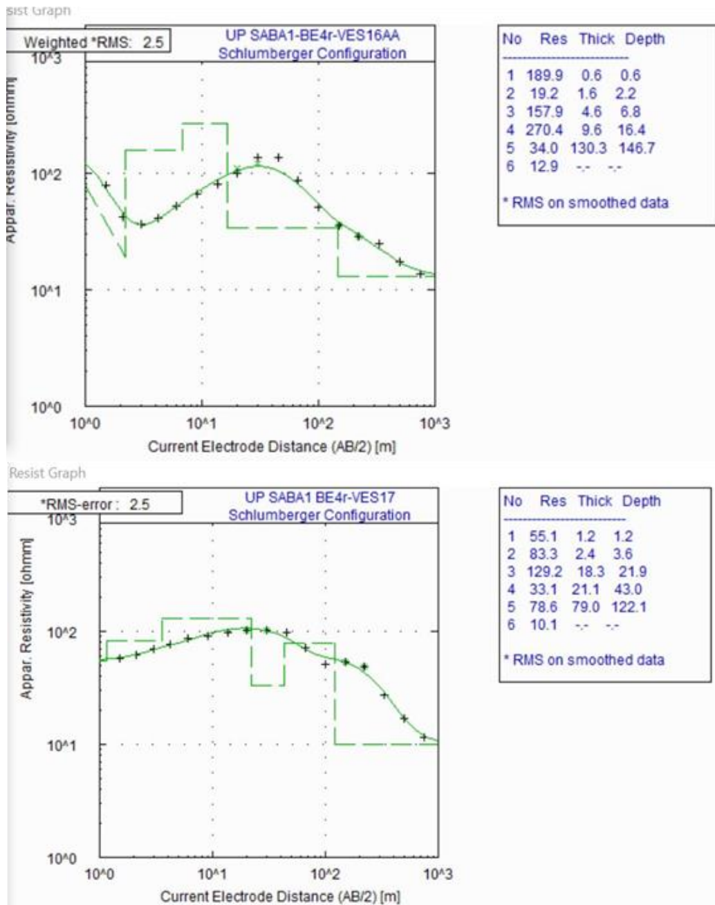
Figure 5.20. Model parameters of the two VES points recommended for drilling points in the central part of BE4r of Berehale Woreda.
