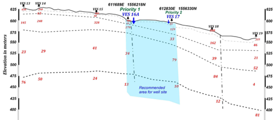
Figure 5.19. Geo-electric sections along a line connecting 8 VES points in the central part of BE4r of Berehale Woreda.
