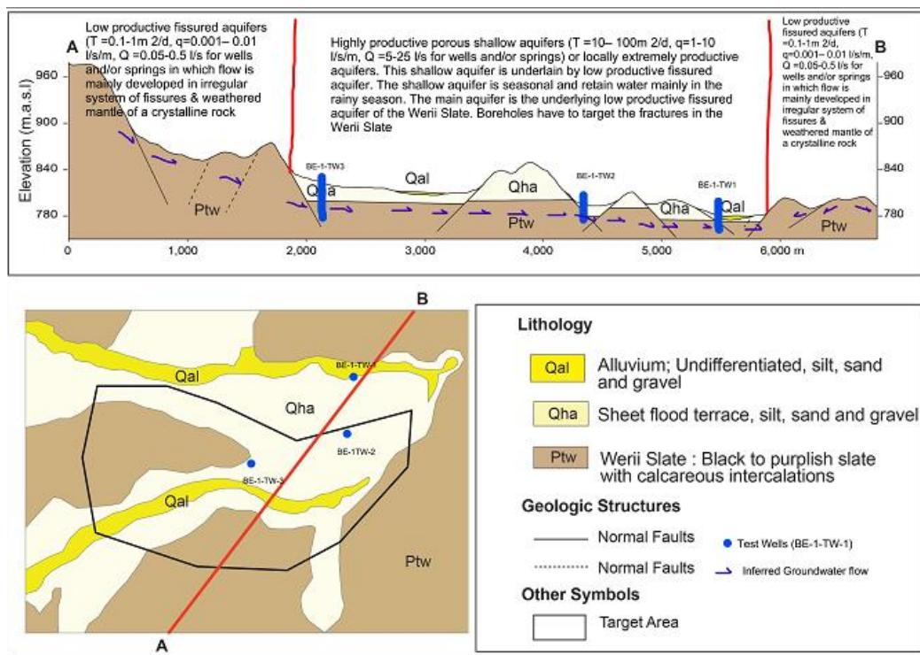
Figure 7.3. Conceptual model for target area Berhale BE1.
