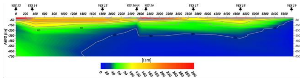
Figure 5.18. Apparent resistivity pseudo depth sections along a line connecting 8 VES points in the central part of BE4r of Berehale Woreda.
