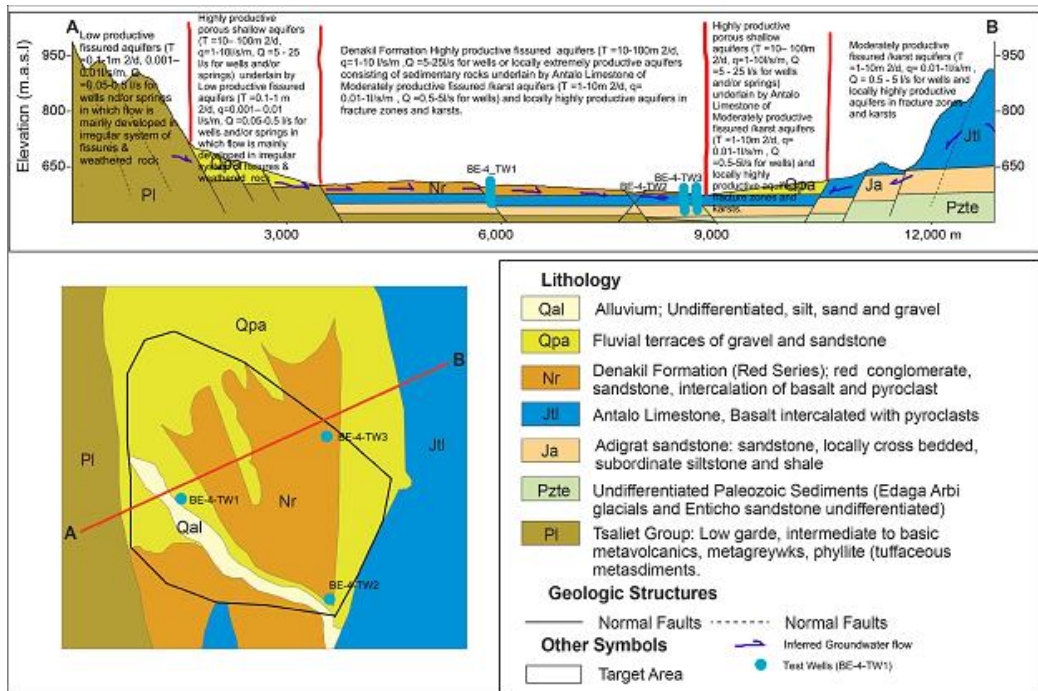
Figure 7.2. Conceptual model for target area Berhale BE4-r.
