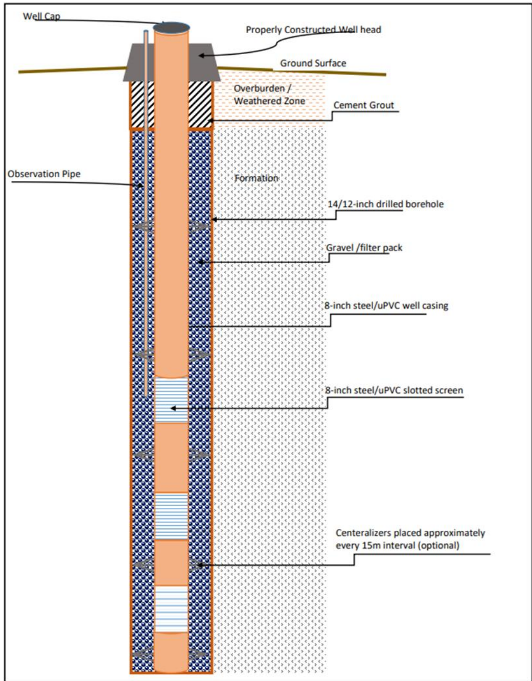
Figure 9.1. Generic well design for Berhale woreda.
