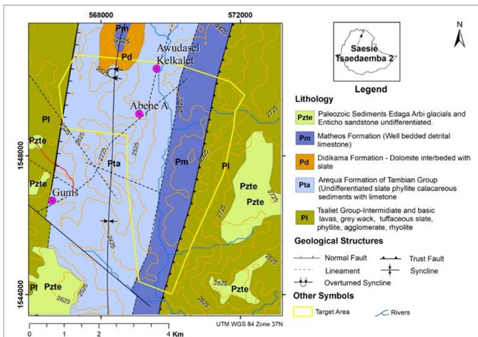
Figure 4.3. Geological map of target area 2 of the Saesi Woreda.
