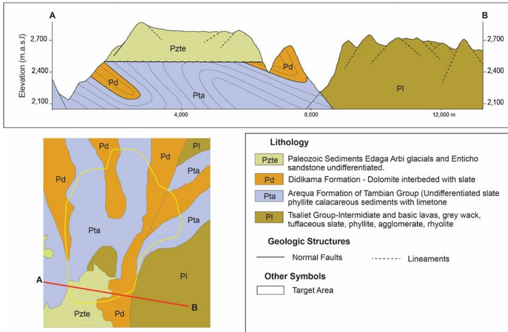
Figure 4.2. Geological cross section of target area 1 of the Saesi Woreda.
