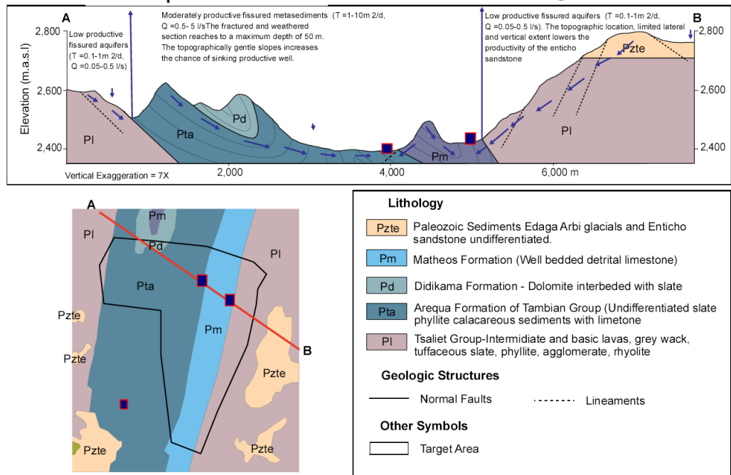
Figure 7.2. Conceptual model for target area Saesie ST3.
