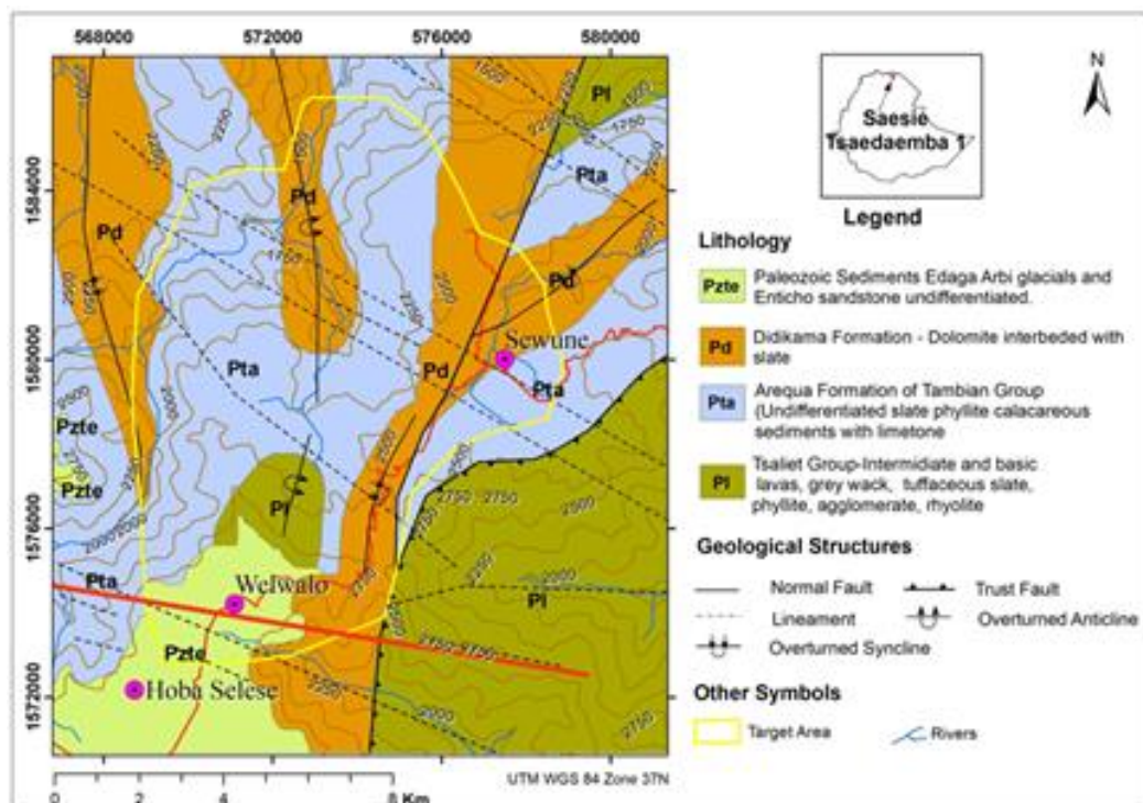
Figure 4.1. Geological map of target area 1 of the Saesie Woreda.
