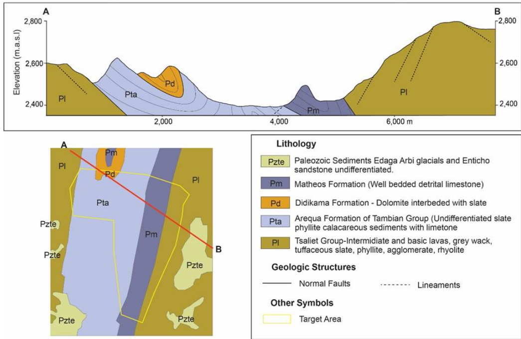
Figure 4.4. Geological cross section across target area 2 of the Saesi Woreda.
