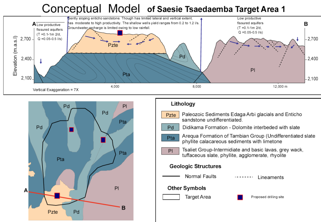
Figure 7.1. Conceptual model for target area Saesie ST2.
